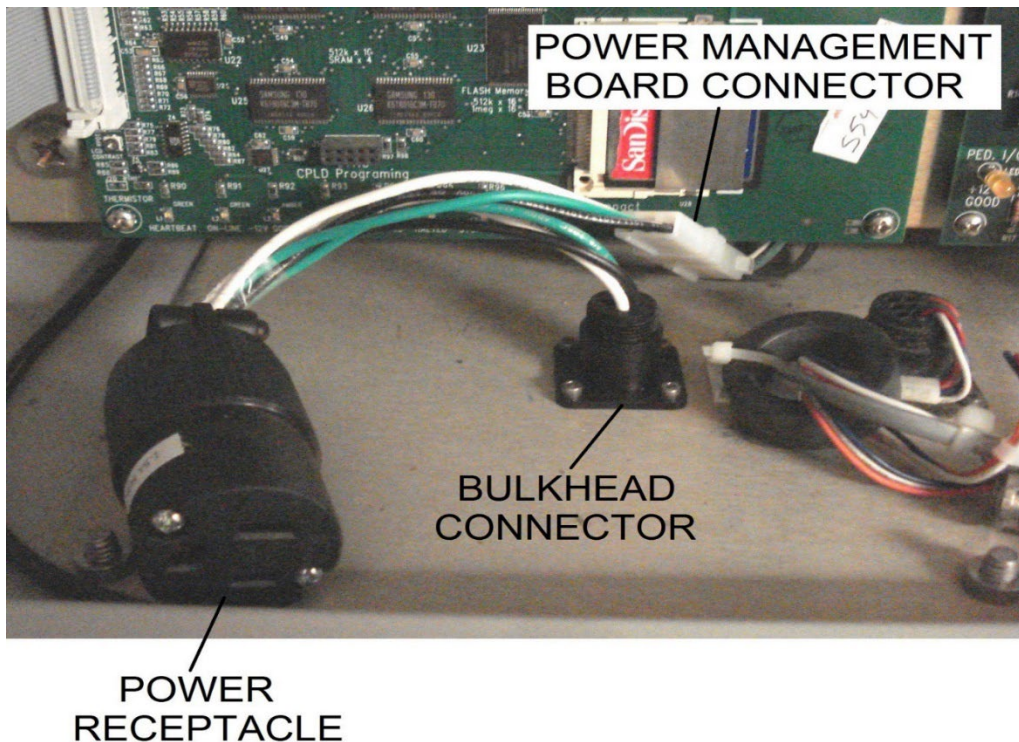
Figure 2. 178802A Cable Installed
