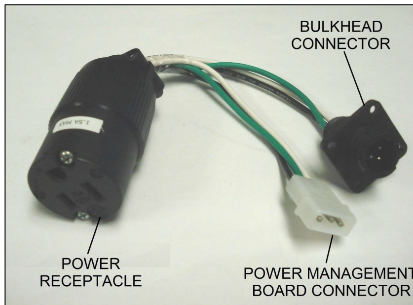
Figure 1. 178802A Cable with Power Receptacle
